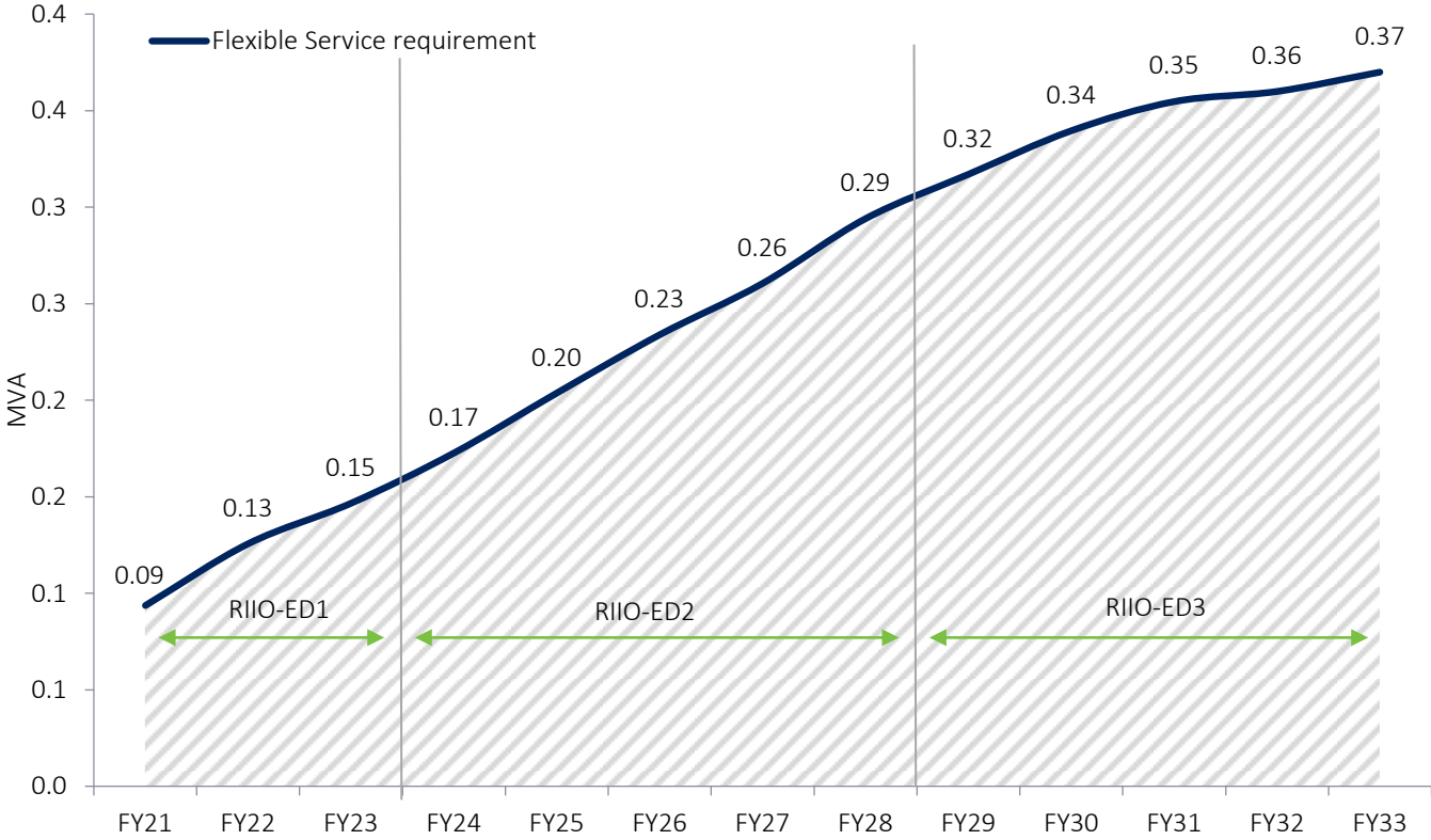
Figure 2.3.3: Forecasted flexible service requirement up to FY33
