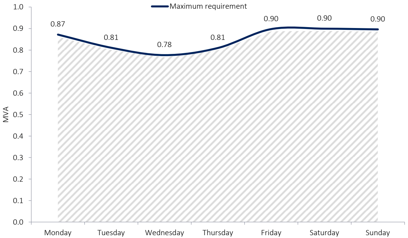
Figure 2.1.5: Maximum estimated flexible service requirement by week day for FY21
