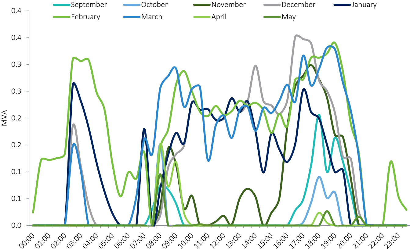
Figure 2.2.6: Estimated time profiled flexible service requirement by month for FY21
