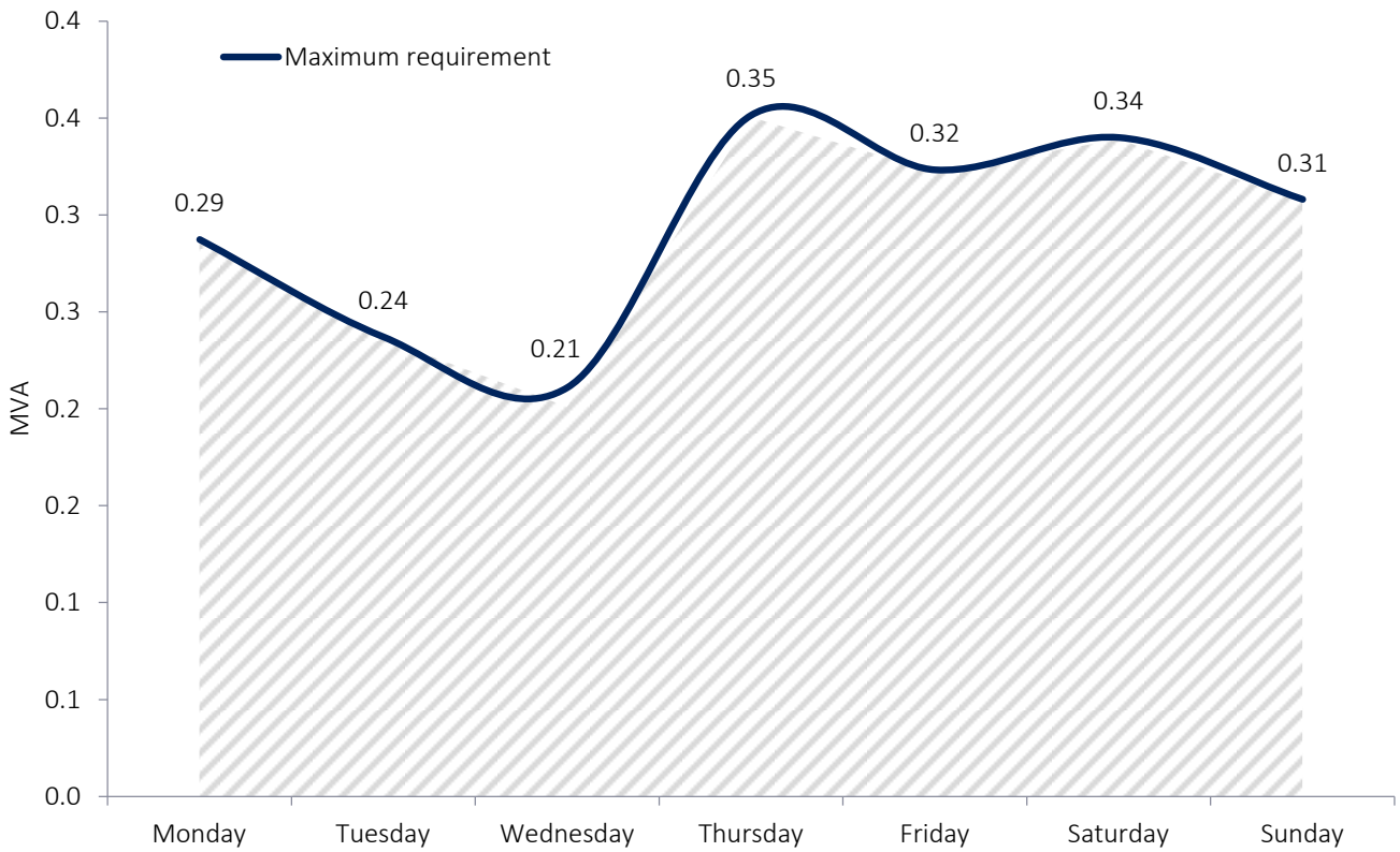
Figure 2.2.5: Maximum estimated flexible service requirement by week day for FY21
