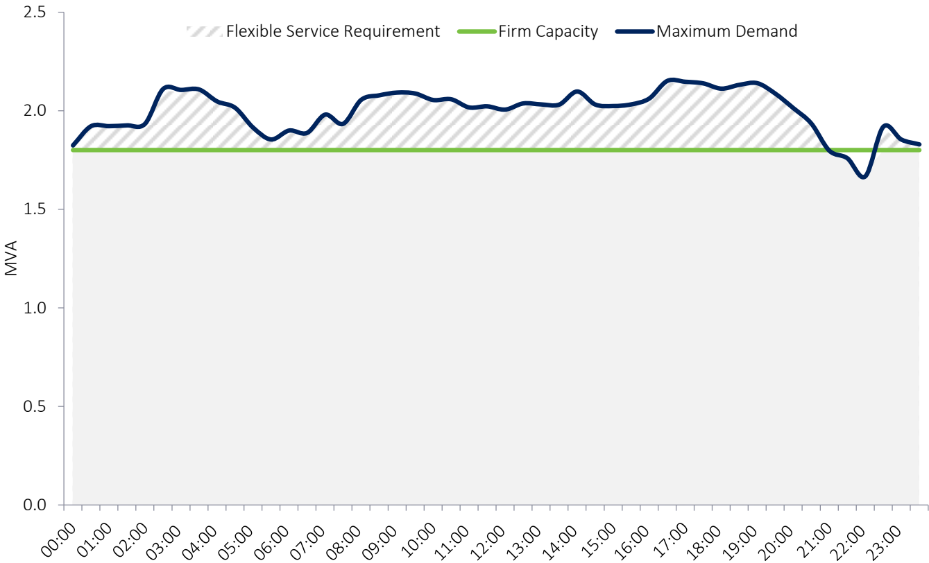
Figure 2.2.2: Estimated maximum daily profile for FY21
