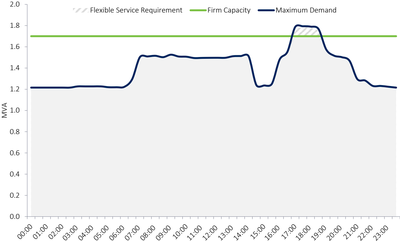
Figure 2.3.2: Estimated maximum daily profile for FY21
