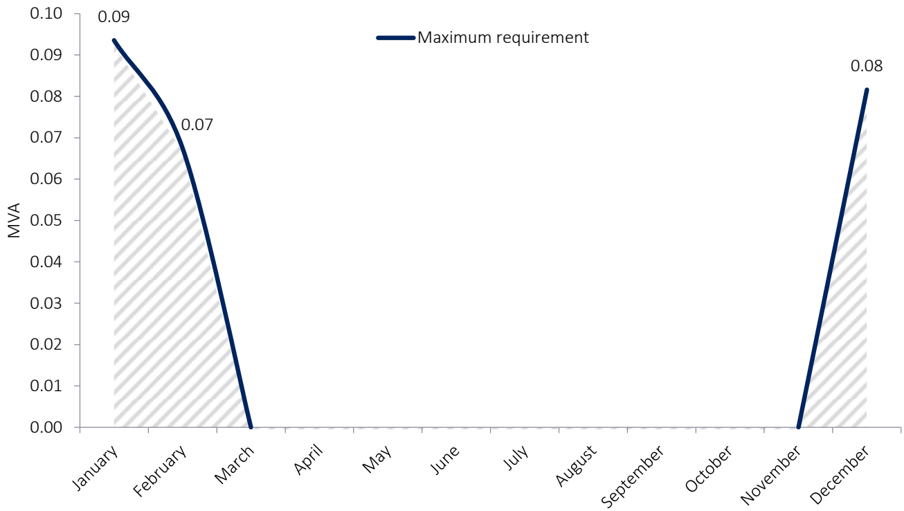
Figure 2.3.4: Maximum estimated flexible service requirement by month for FY21
