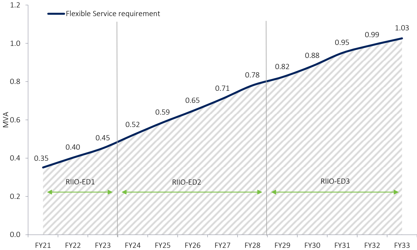
Figure 2.2.3: Forecasted flexible service requirement up to FY33
