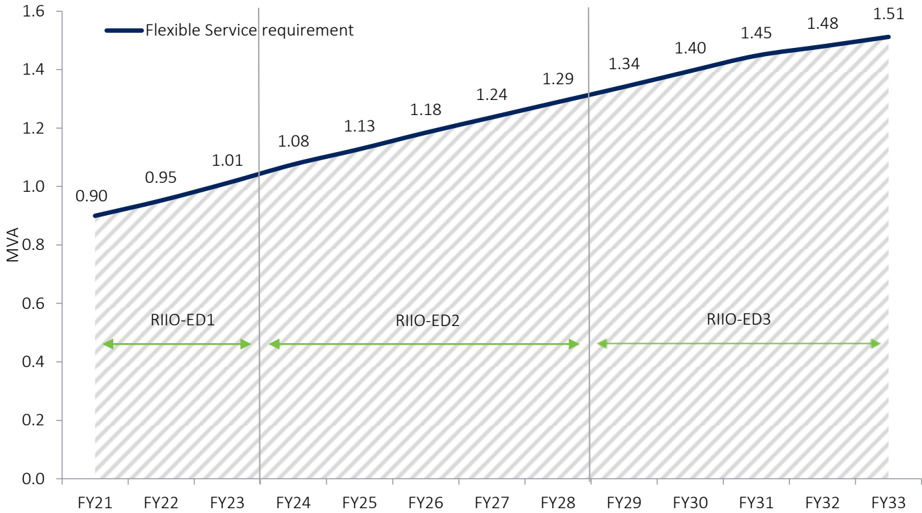
Figure 2.1.3: Forecasted flexible service requirement up to FY33
