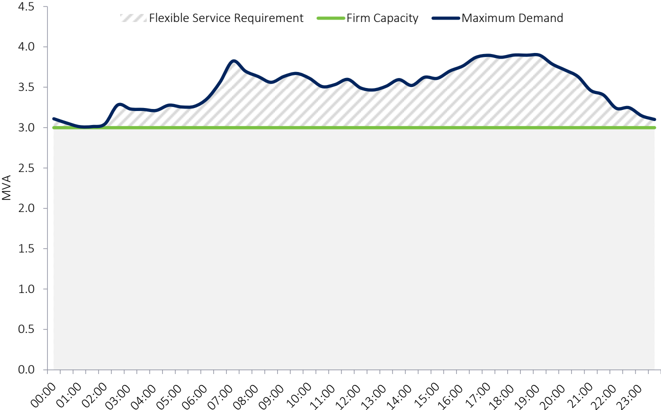
Figure 2.1.3: Forecasted flexible service requirement up to FY33
