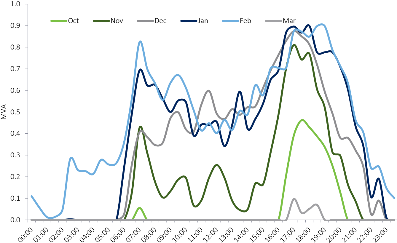
Figure 2.1.6: Estimated time profiled flexible service requirement by month for FY21
