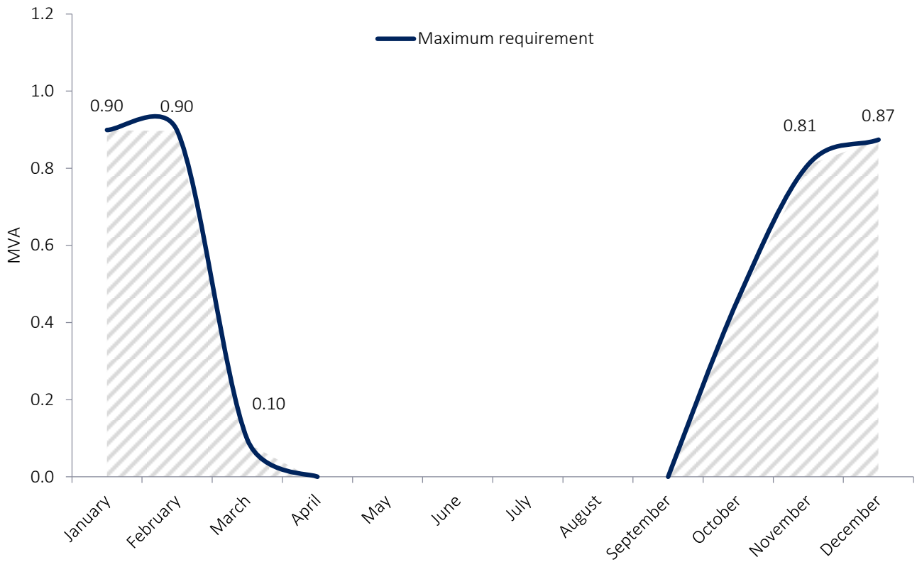
Figure 2.1.4: Maximum estimated flexible service requirement by month for FY21
