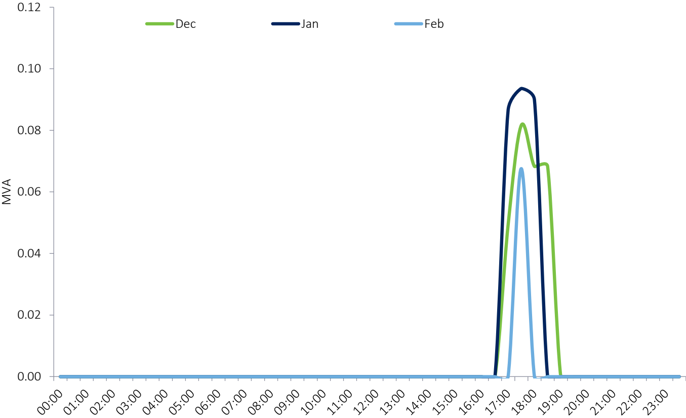
Figure 2.3.6: Estimated time profiled flexible service requirement by month for FY21
